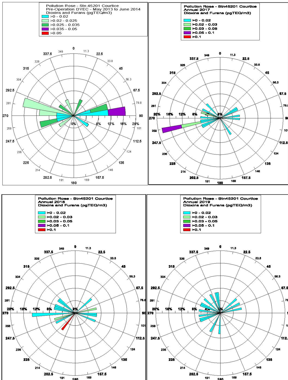
Figure C5 Dioxins and Furans 24-hour Average Pollution Roses – DYEC Monitoring Program - Courtice
