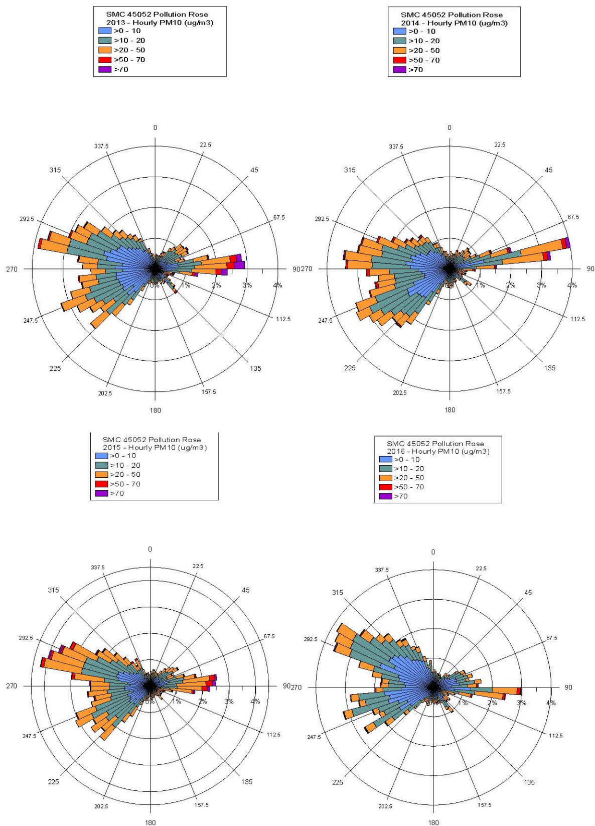
Figure C7 PM 10 Hourly Pollution Roses– St. Mary's Cement Monitoring Program - SMC1 (45052)
