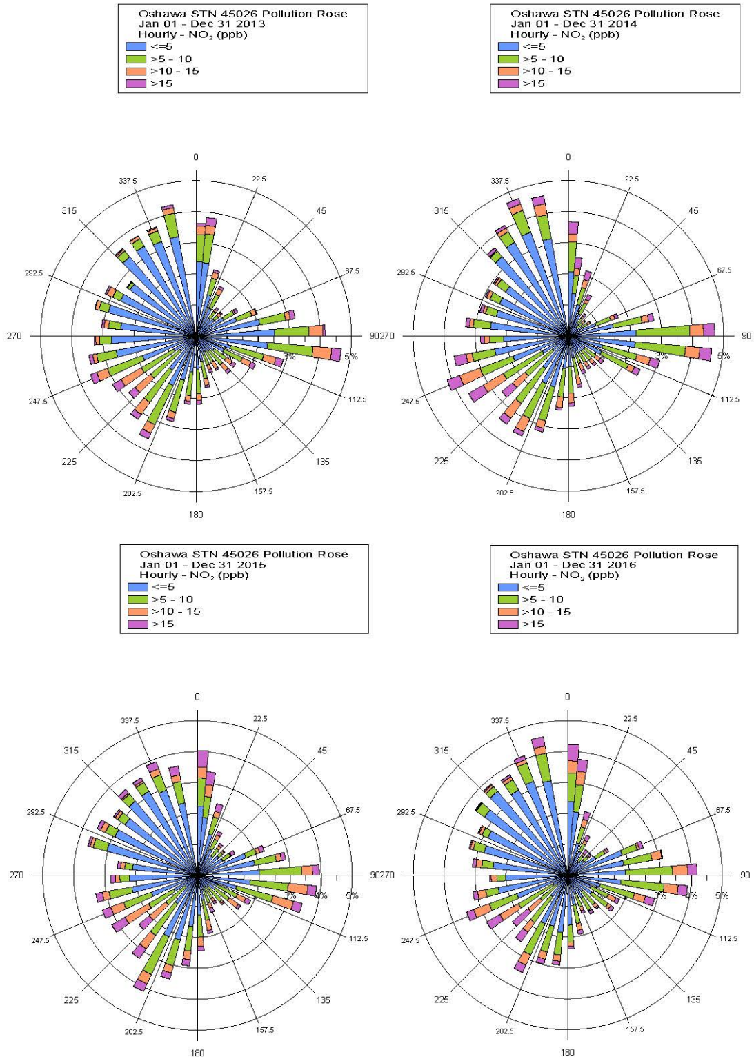
Figure C14 Hourly NO 2 Pollution Roses – Oshawa AQHI Station
